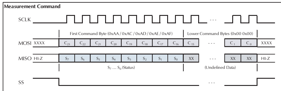
Figure 4 - SPI Communications Diagram
