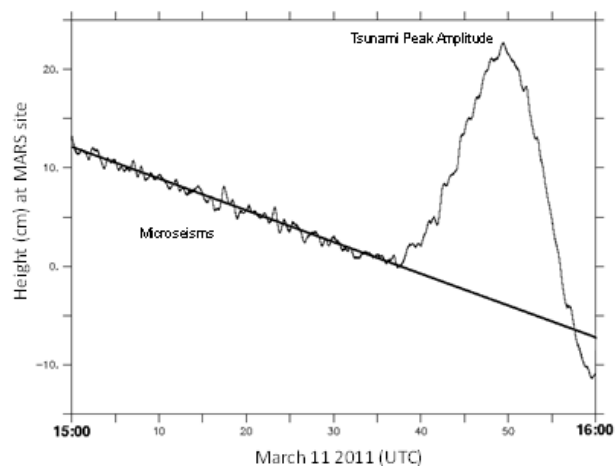
Figure 6. Nano-resolution pressure sensor at 40 Hz measures a 25 cm tsunami wave in Monterey Bay, California, which was a result of the Honshu, Japan earthquake on March 11, 2011.
